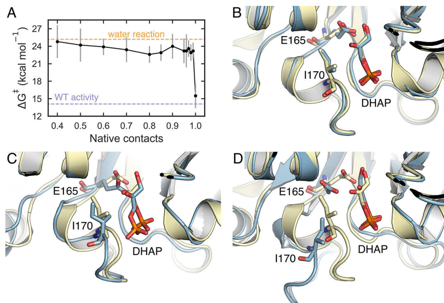
Figure 7. (A) Activation free energies obtained from EVB simulations of TIM at different conformations of loop 6, based on structures extracted from our BE-METAD simulations, as described in the main text. Data points show averages and standard deviations (as error bars) over 50 individual EVB trajectories per Q value. The corresponding raw data are shown in Table S8. (B–D) Comparison of the crystal structure of TIM with loop 6 in a closed conformation (PDB ID: 1NEY, 16,35 yellow) with representative starting structures from our BE-METAD simulations (blue), at native contacts of (B) Q = 1.00 , (C) Q = 0.99 , and (D) Q = 0.40 . For structural overlays of all 10 structures used for the EVB simulations at each Q value, see Figure S16. For a description of how the structures were selected, see the main text.
