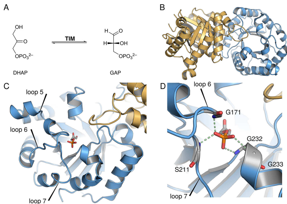
Figure 1. (A) Scheme showing the interconversion of DHAP and GAP. (B) Overall structure of \gamma TIM (PDB ID: 1NEY), 16,35 highlighting also (C) loops 5, 6, and 7 and (D) the stabilization of the phosphodianion of the substrate DHAP by four discrete H-bonds formed with the protein backbone.
